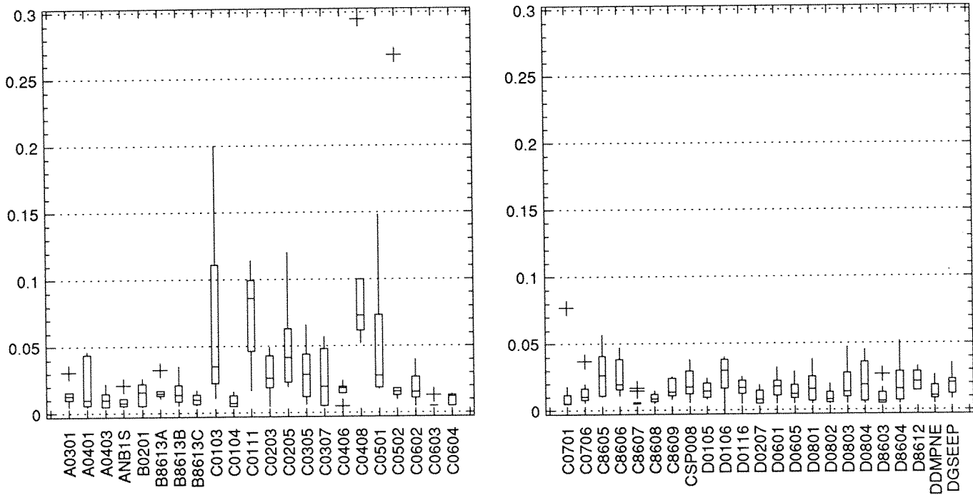
Figure 3-10. Total Organic Halogens (mg/L) in Groundwater Samples from the Sand and Gravel Unit
