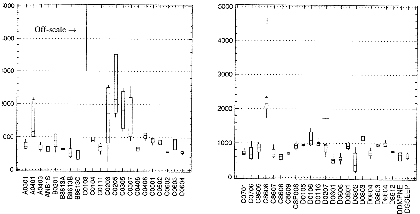
Figure 3-8. Conductivity ( \mu\text{mhos}/\text{cm}@25^{\circ} ) from the Sand and Gravel Unit (Note: well WNW0103 is off-scale.)
