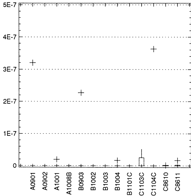
Figure 3-34. Tritium Activity ( \mu\text{Ci}/\text{mL} ) in Groundwater Samples from the Lacustrine Unit
