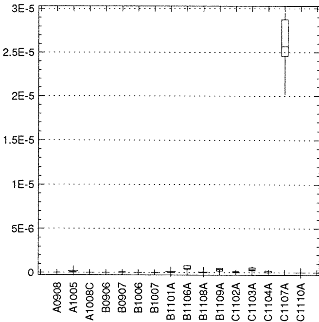
Figure 3-41. Tritium Activity ( \mu\text{Ci}/\text{mL} ) in Groundwater Samples from the Weathered Lavery Till Unit
