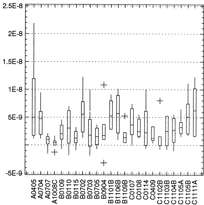
Figure 3-25. Gross Alpha ( \mu\text{Ci}/\text{mL} ) in Groundwater Samples from the Unweathered Lavery Till Unit
