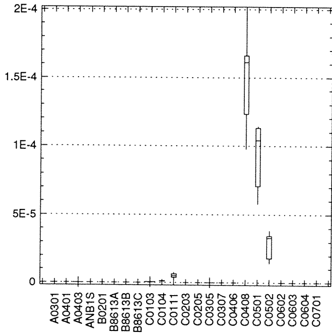
Figure 3-12. Gross Beta ( \mu\text{Ci/mL} ) in Groundwater Samples from the Sand and Gravel Unit
