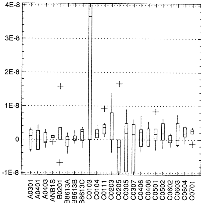
Figure 3-11. Gross Alpha ( \mu\text{Ci/mL} ) in Groundwater Samples from the Sand and Gravel Unit
