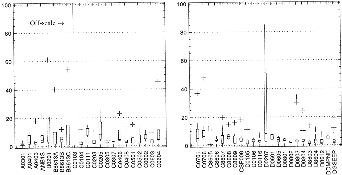
Figure 3-9. Total Organic Carbon (mg/L) in Groundwater Samples from the Sand and Gravel Unit
