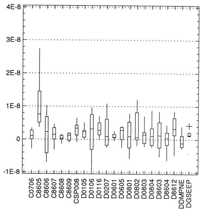
Figure 3-11. Gross Alpha ( \mu\text{Ci/mL} ) in Groundwater Samples from the Sand and Gravel Unit
