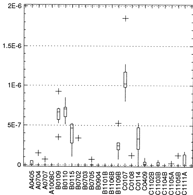
Figure 3-27. Tritium activity ( \mu\text{Ci}/\text{mL} ) in Groundwater Samples from the Unweathered Lavery Till Unit
