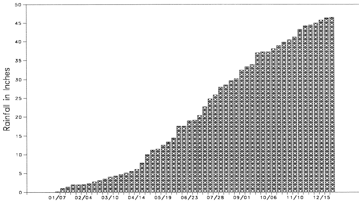
Figure C - 6.4. 1992 Cumulative Rainfall
